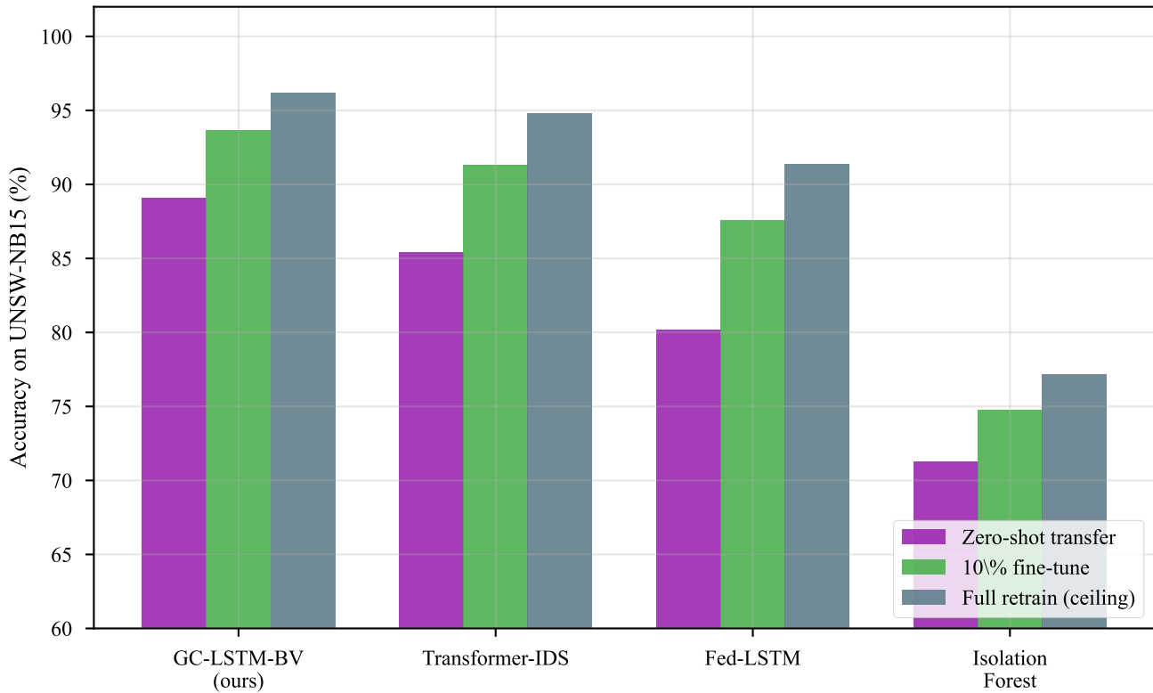
Cross-Domain Validation: V2G \rightarrow UNSW-NB15 Real-World Attacks
